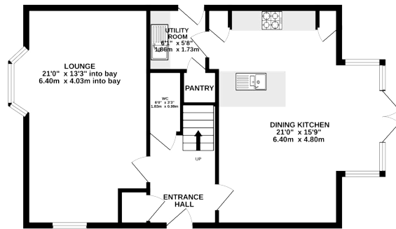
GROUND FLOOR 685 sq.ft. (63.7 sq.m.) approx.
